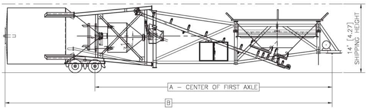
DC-COLT - TOWING POSITION
